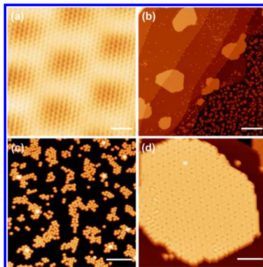
Figure 1. (a) Atomic-resolution STM image of graphene on Ir(111). (b) STM image showing both the \text{C}_{60}/\text{Ir}(111) (lower right) and \text{C}_{60}/\text{graphene}/\text{Ir}(111) (upper left) regions. (c) STM image of small \text{C}_{60} clusters formed on Ir(111). (d) STM image of large \text{C}_{60} islands formed on graphene/Ir(111). Scanning parameters: (a) V_{\text{bias}} = 20 \text{ mV} , I = 8 \text{ nA} ; (b) V_{\text{bias}} = 3 \text{ V} , I = 10 \text{ pA} ; (c) V_{\text{bias}} = 2 \text{ V} , I = 100 \text{ pA} ; and (d) V_{\text{bias}} = 3 \text{ V} , I = 50 \text{ pA} . Scale bars: (a) 1; (b) 50; (c) 10; and (d) 10 nm.
