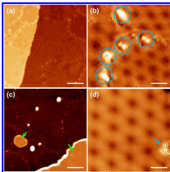
Figure 6. STM images of graphene obtained by thermal annealing 0.7 ML C_{60} molecules on Ir(111). (a) Different graphene domains with varied moiré patterns coexist in the graphene layer. (b) Atomic-resolution STM image of the boundaries between three different graphene domains. The graphene lattices in these three domains are different from each other, leading to different moiré patterns. (c) Bilayer graphene islands formed on the surface. (d) Atomic-resolution STM image of the bilayer graphene. The feature indicated by the arrow is the electron-scattering pattern around a defect. Scanning parameters: (a) V_{\text{bias}} = 3 V, I = 50 pA; (b) V_{\text{bias}} = 10 mV, I = 5 nA; (c) V_{\text{bias}} = 2 V, I = 50 pA; and (d) V_{\text{bias}} = 10 mV, I = 5 nA. Scale bars: (a) 13; (b) 2; (c) 16; and (d) 2 nm.
