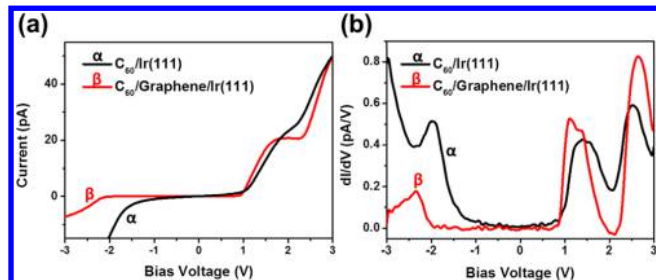
Figure 2. STS of C_{60} molecules on Ir(111) and graphene/Ir(111) surfaces. Stabilization conditions: V_{\text{bias}} = 3 V, I = 50 pA.
