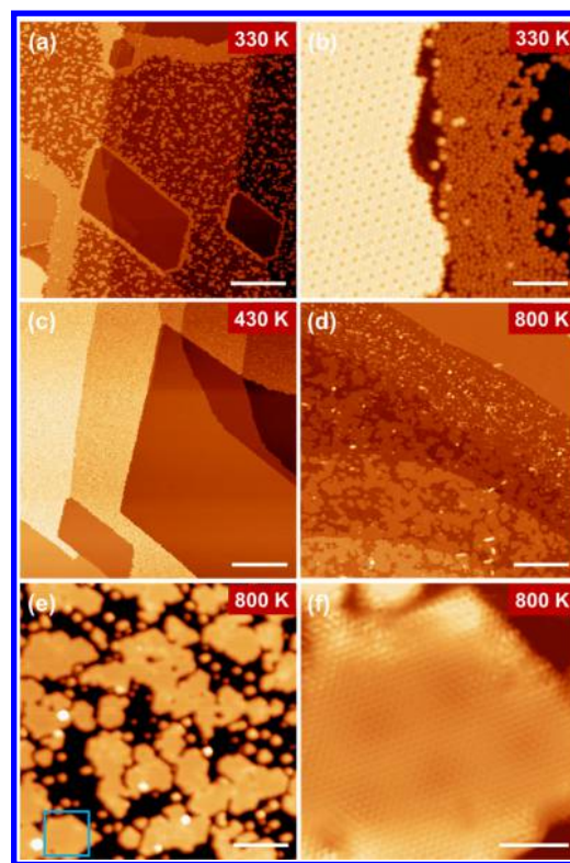
Figure 3. STM images of the C_{60} /Ir(111) and C_{60} /graphene/Ir(111) regions after thermal annealing at (a,b) 330 K for 30 min, (c) 430 K for 30 min, and (d–f) 800 K for 30 min. The atomic-resolution STM image in panel f was recorded in the region indicated by the square in panel e. Scanning parameters: (a–d) V_{\text{bias}} = 3 V, I = 50 pA; (e) V_{\text{bias}} = 2 V, I = 50 pA; and (f) V_{\text{bias}} = 10 mV, I = 9 nA. Scale bars: (a) 40; (b) 10; (c) 40; (d) 40; (e) 10; and (f) 2 nm.
