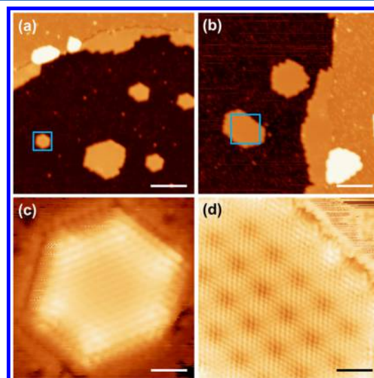
Figure 5. STM images of graphene patches obtained by thermal annealing 0.1 ML C_{60} molecules on Ir(111). The atomic-resolution STM images in panels c and d were recorded in the regions marked with a square in panels a and b, respectively. Different orientations of graphene lattice were observed for the graphene patches, as demonstrated by the atomic-resolution STM images. Scanning parameters: (a) V_{\text{bias}} = 2 V, I = 50 pA; (b) V_{\text{bias}} = 2 V, I = 50 pA; (c) V_{\text{bias}} = 200 mV, I = 5 nA; and (d) V_{\text{bias}} = 100 mV, I = 5 nA. Scale bars: (a) 10; (b) 10; (c) 1; and (d) 1.6 nm.
