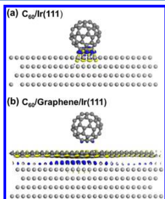
Figure 4. DFT simulations of C_{60} molecules on (a) Ir(111) and (b) graphene/Ir(111). The calculations show a significant charge transfer for C_{60} on Ir(111), while the C_{60} molecules are quasi-free on the graphene/Ir(111) surface with negligible charge transfer.
