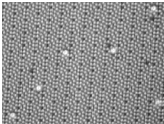
Fig. 3. The STM image shows some GRCs on the Si(111)-(7 × 7) surface. The sample bias and tunnelling current are +1.5 V and 0.4 nA, respectively.
