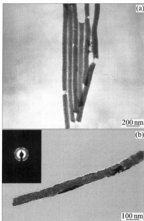
Fig.3 TEM image of dispersed CuO nanowires (a) and single CuO nanowires and corresponding selected area diffraction pattern (b) of nanowires
